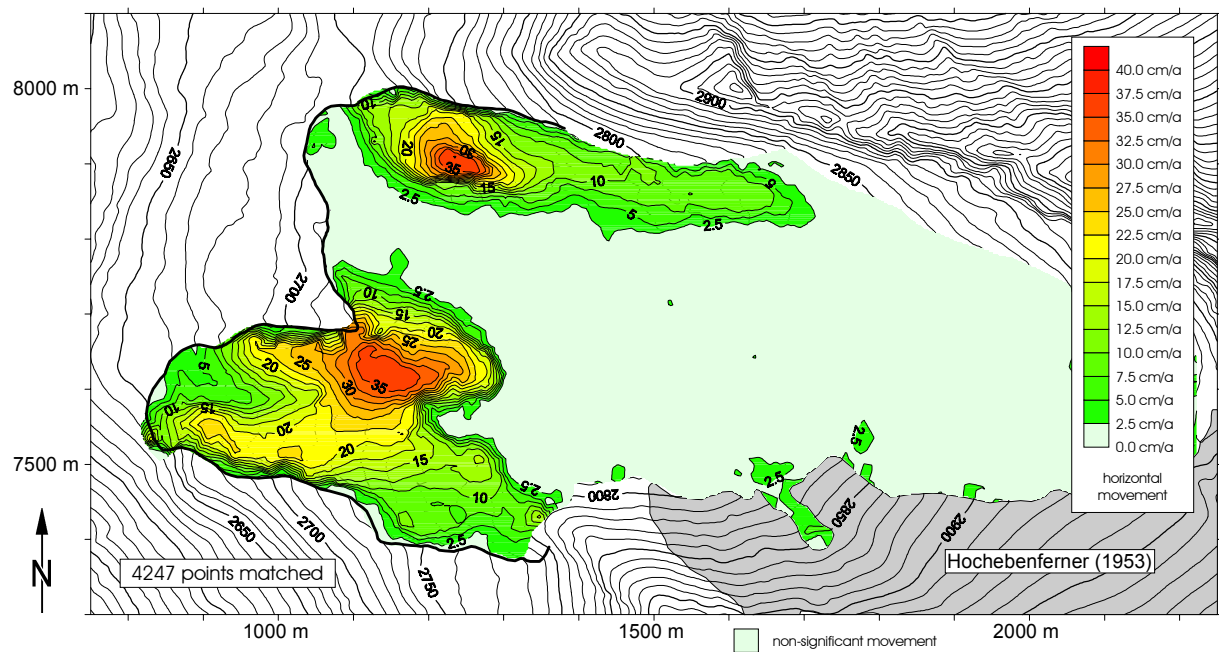
Figure 9: Mean annual horizontal flow velocity at Inner Hochebenkar rock glacier for the time period 1953-1997.
